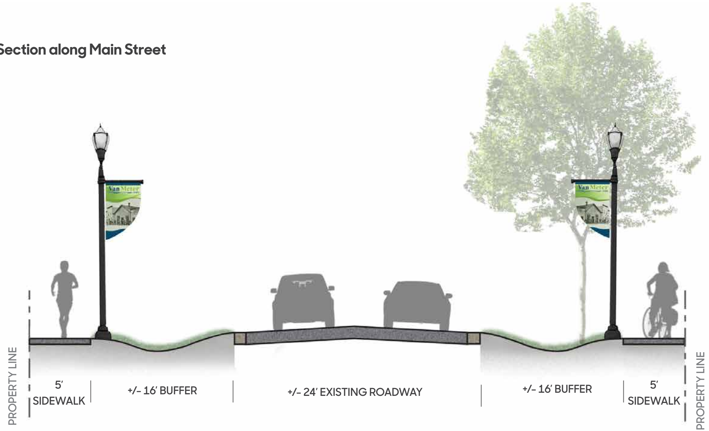
Proposed Main St. corridor improvements
