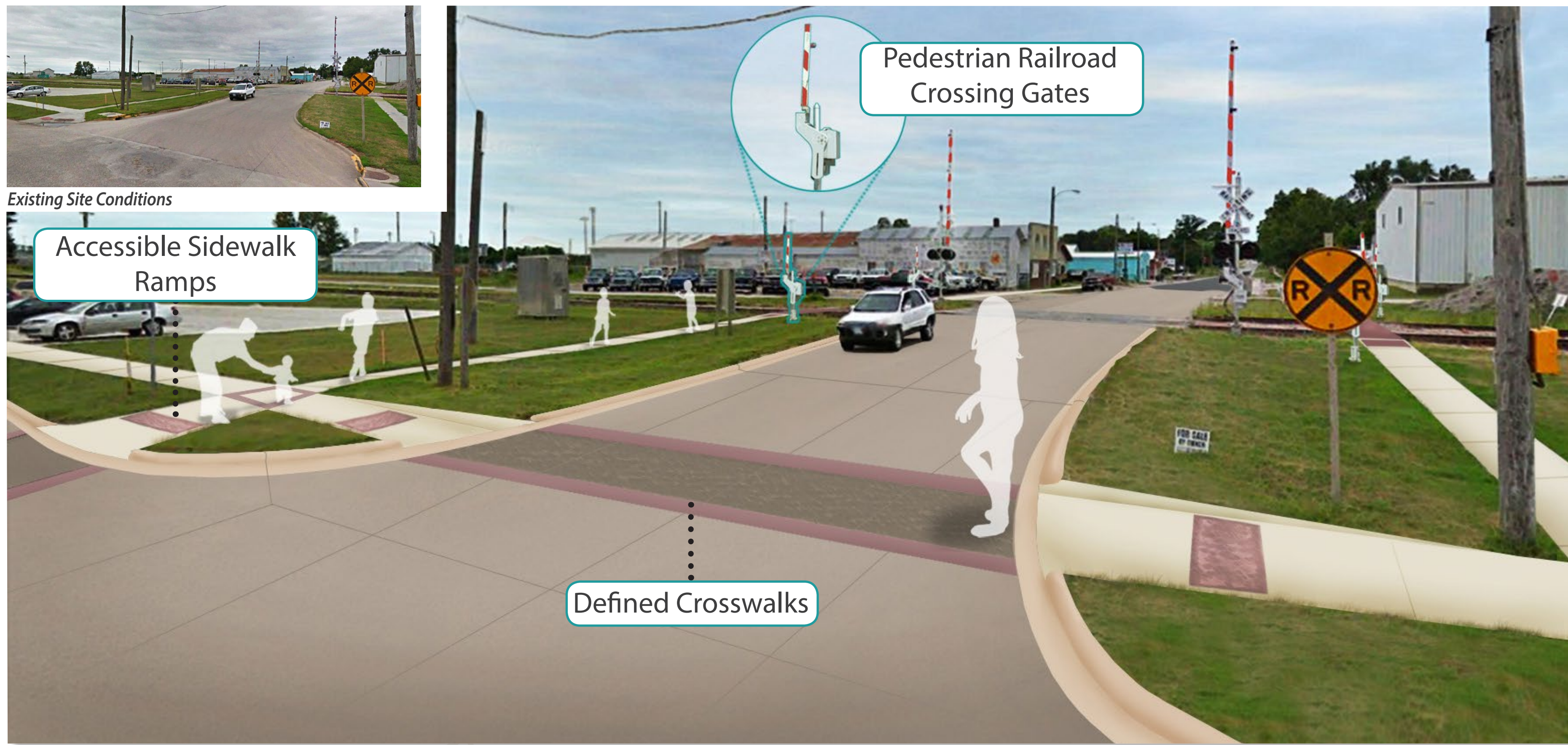
Pedestrian connection improvements along the intersection of 350th (Front) Street and S Division Street including safer railroad crossings.
