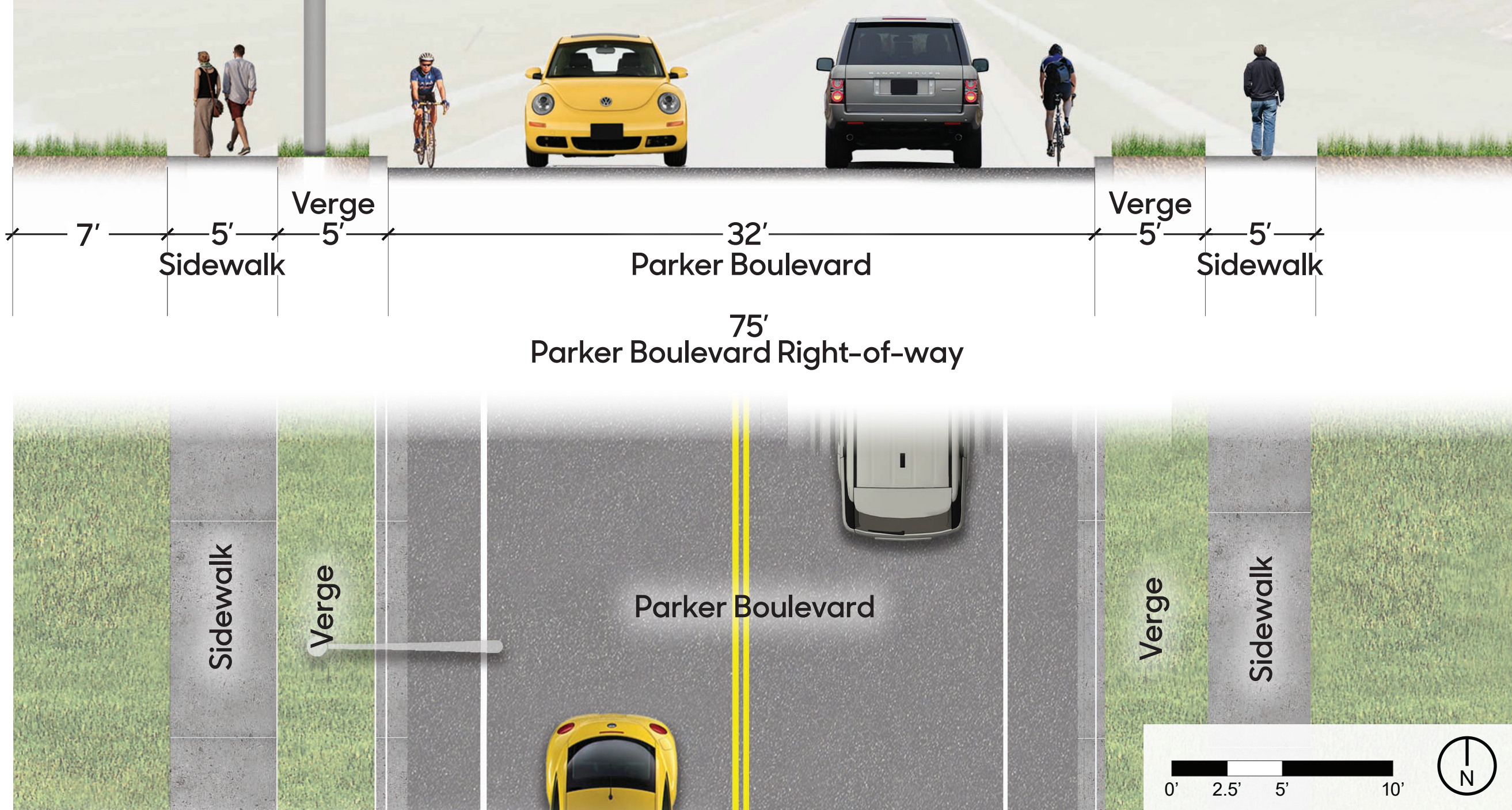
Detail Plan of Existing Conditions Along Parker Boulevard
