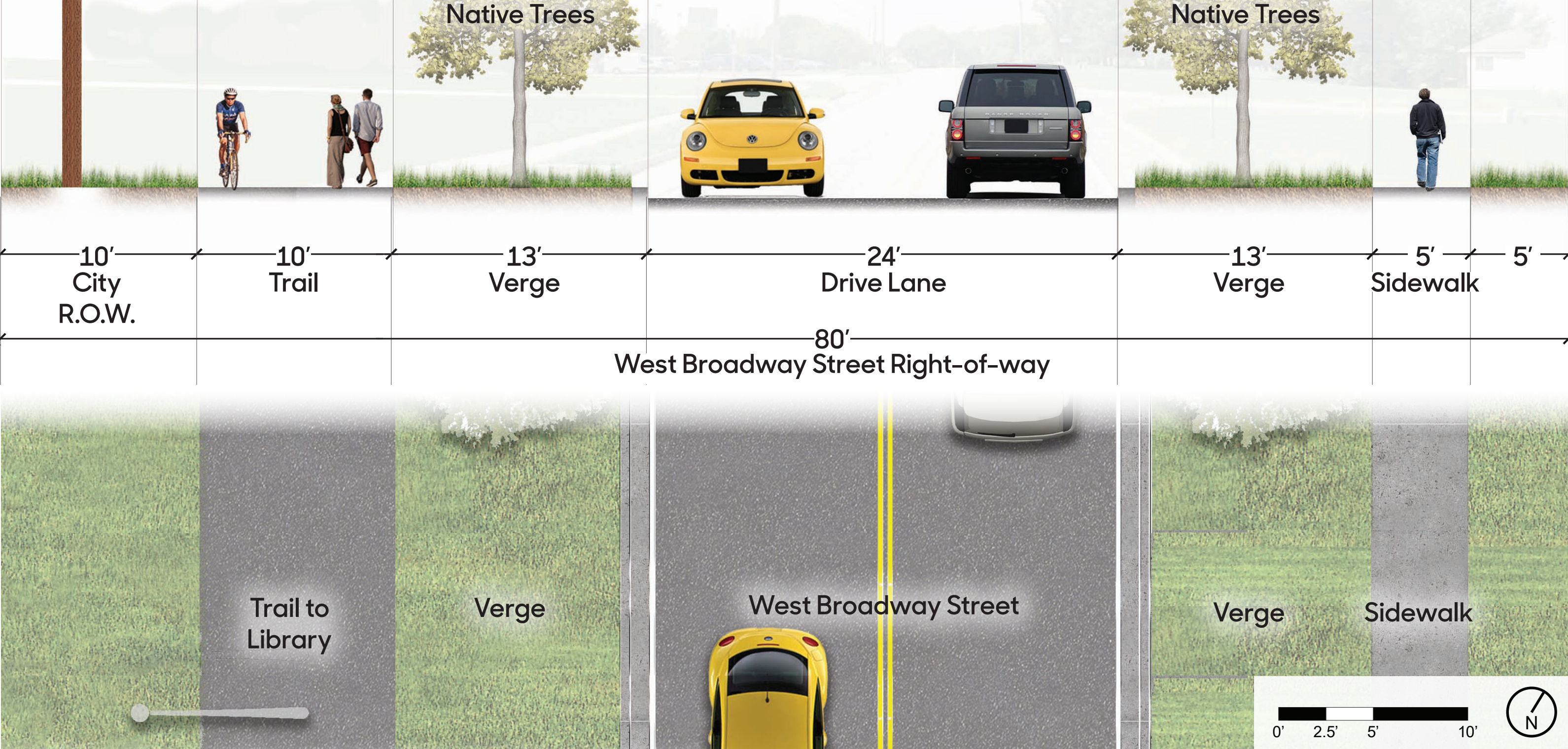
Detail Plan of Proposed Improvements Along West Broadway Street
