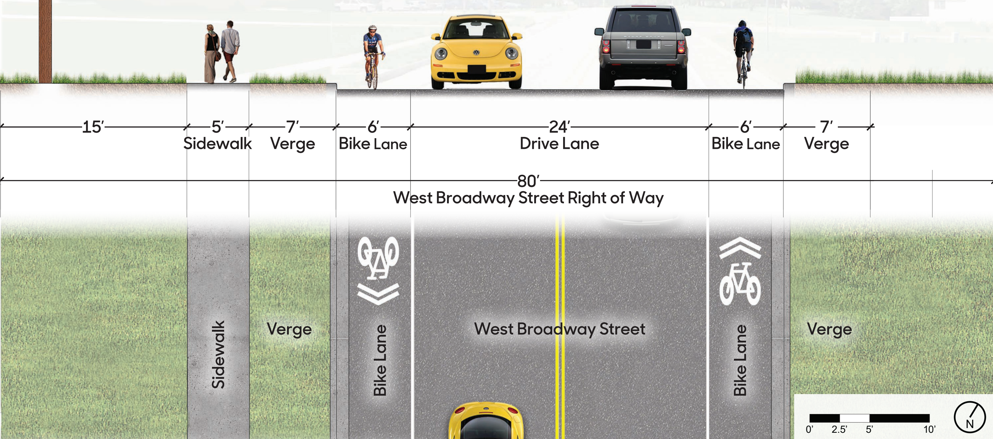
Detail Plan of Existing Conditions Along West Broadway Street
