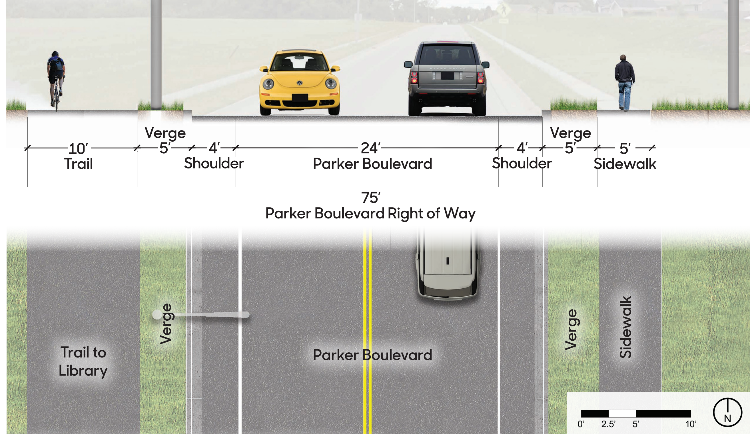
Detail Plan of Proposed Improvements Along Parker Boulevard
