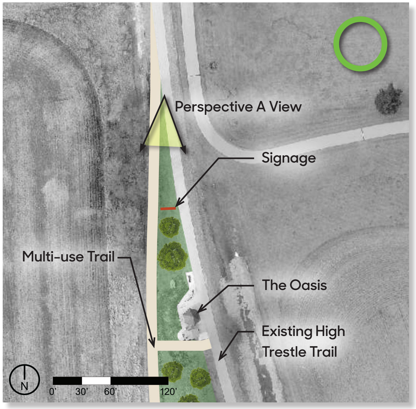
Polk City Trail at The Oasis Detail Plan
