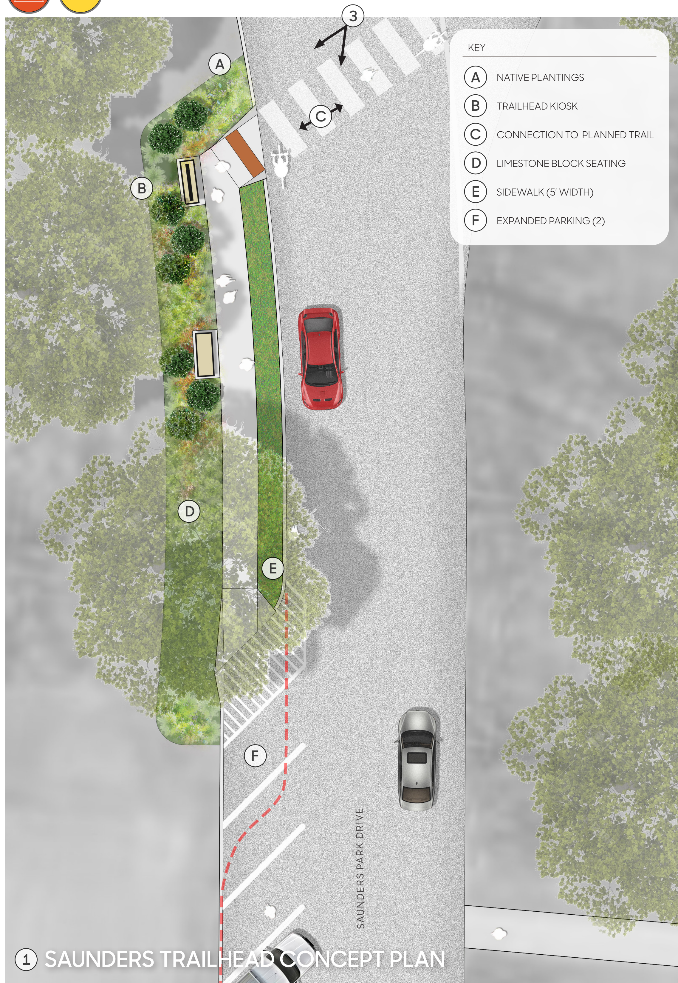
1 SAUNDERS TRAILHEAD CONCEPT PLAN Plan view showing the proposed trailhead monument, connections, and amenities. The trailhead is planned as a pass-through space highlighting the beauty of its setting
