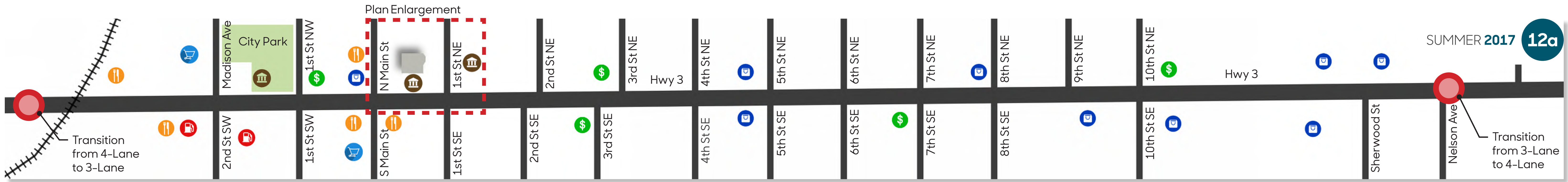
4-lane Highway 3 corridor plan showing where the proposed 3-lane transitions occur
