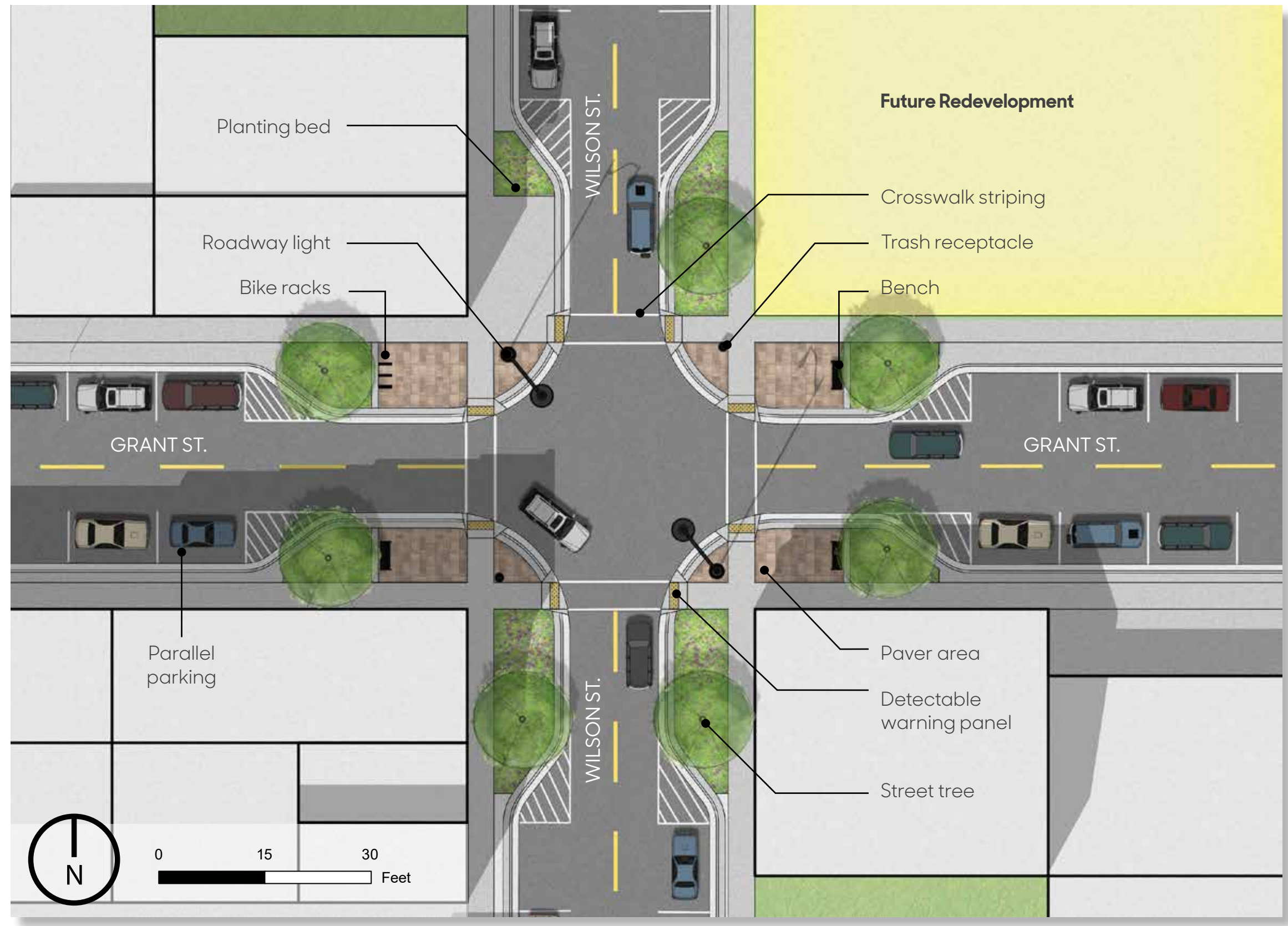
Plan enlargement at intersection of Grant St. and Wilson St.
